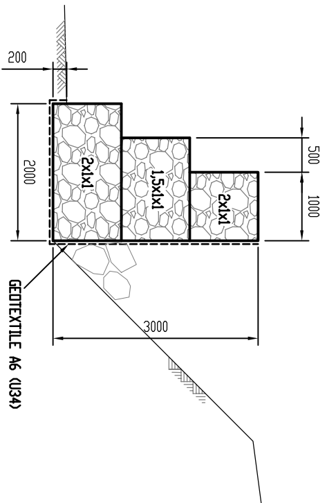
3m HIGH GABION CATCH WALL
